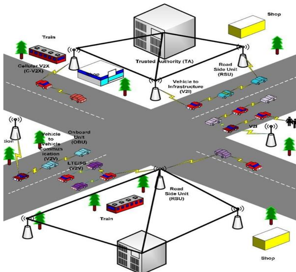
Figure 1: VANET
