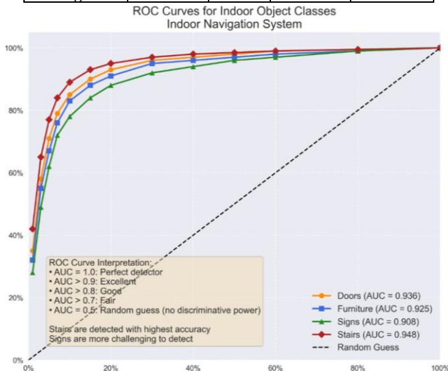
Figure 4.2: Roc curve
