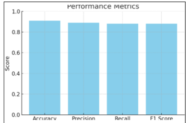
Figure 1: Performance Metrics
