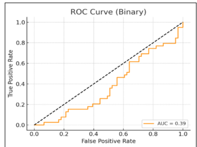
Figure 2: ROC Curve
