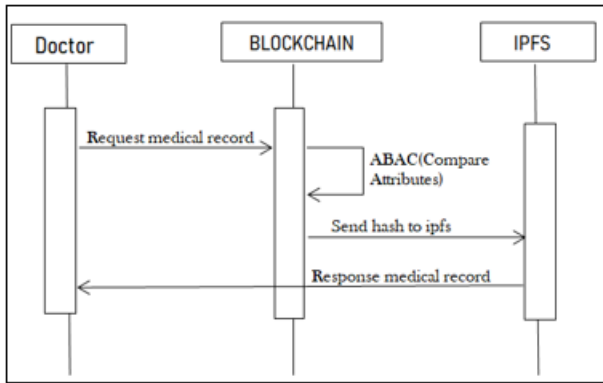
Figure 3: Data Access from Blockchain
