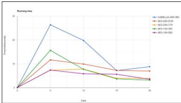
Figure 5: Time complexity
