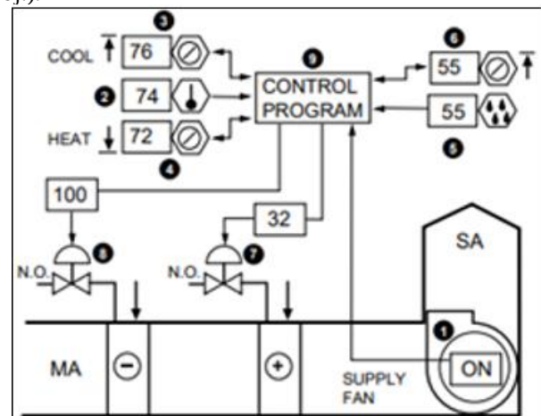
Figure 1: BAS Dehumidification Control Process
