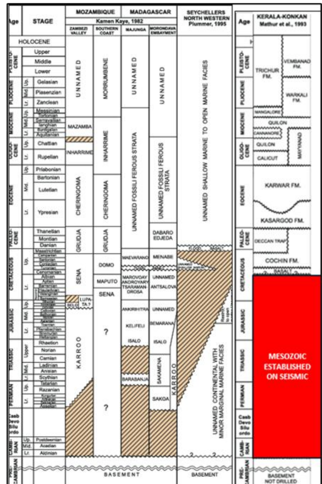
Figure 4a: Stratigraphy of palaeogeographic associates of Kerala Konkan Basin 6 and Figure 4b: Postulated Stratigraphy of Kerala Basin 7
