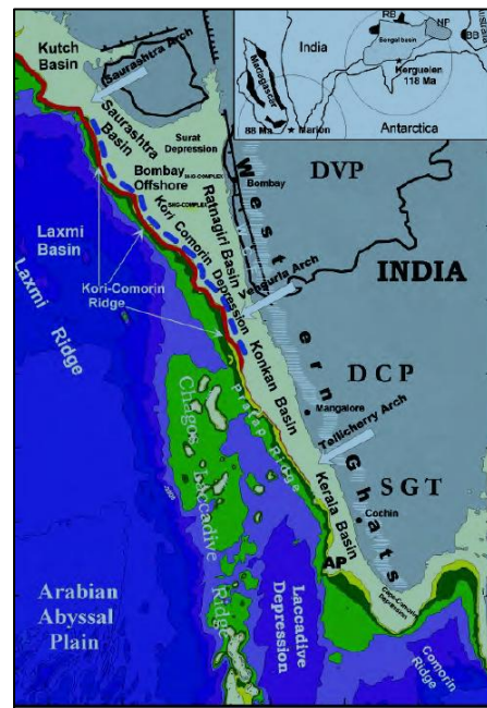
Figure 1: Tectonic map of the western coastal margin of India 3
