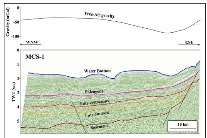
Figure 12: Multi-channel seismic profiles (MCS1) of the Mannar basin along with free-air gravity anomalies derived from the gravity grid along these profiles 9
