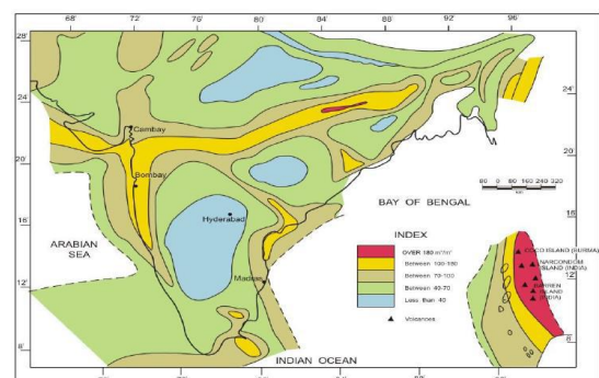
Figure 9: Heat flow map of India and adjoining areas 22
