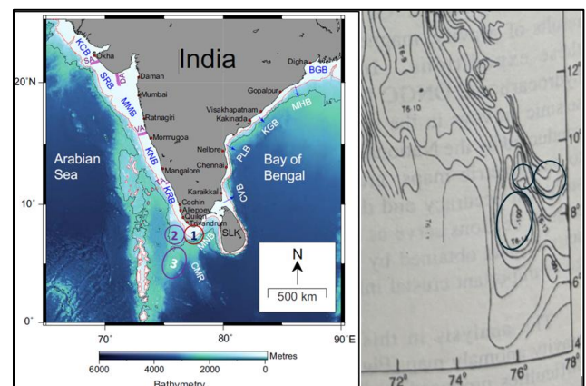
Figure 17: Bathymetry map 33 and Bouguer gravity anomaly map 34 with areas that merit attention by drilling
