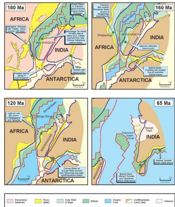
Figure 6: Distribution of regional source rocks; paleogeographic reconstructions for 180, 160, 120, and 65 mega annum 9 .
