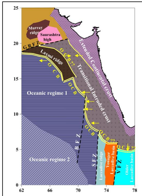
Figure 15: Illustrates the inferred crustal structure, the continental-oceanic boundary (COB), and various spreading regimes in the western offshore region 31 .
