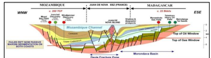
Figure 11: Geological cross-section illustrating the area from the Rovuma Basin in Mozambique to the coastal region of Madagascar, providing context for the recent findings in the Rovuma delta 27
