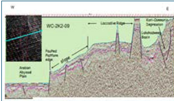
Figure 2: Regional line showing the tectonic elements 1
