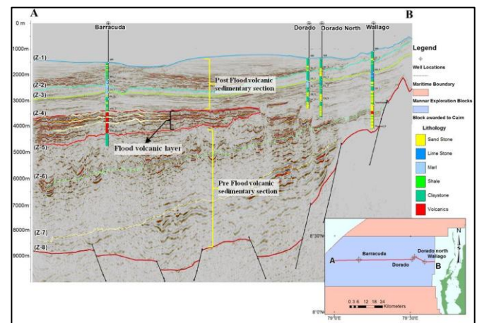
Figure 14: Seismic profile in depth through the recent wells (from A-B in the base map) 29
