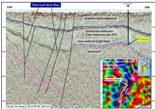
Figure 10: Illustrates the oil indications at Ile Saint Marie-1 on a strike line oriented from SSW to NNE, along the eastern margin of Madagascar. An accompanying inset highlights areas of low gravity, represented in blue on the Bouguer gravity map, with the 2D reprocessed seismic survey depicted in black 25 .
