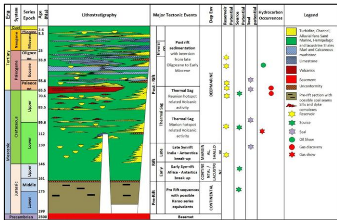
Figure 5: Stratigraphy of Mannar Basin 8
