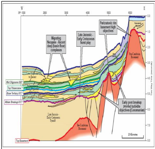
Figure 13: Cartoon illustrating play concepts in Mannar Basin 9
