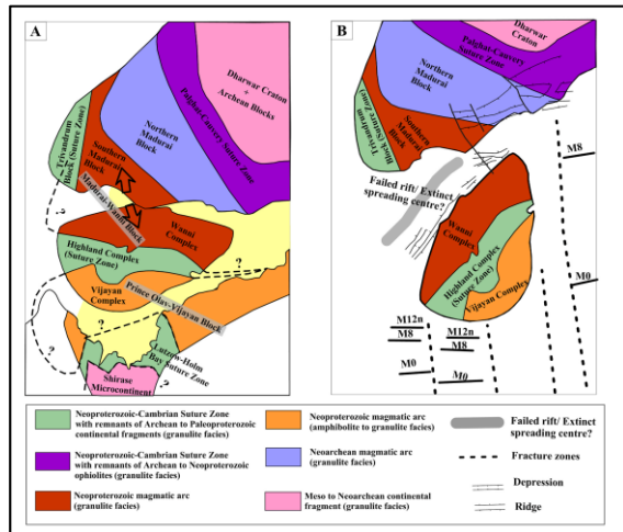
Figure 7: Schematic plate reconstruction models illustrating the evolution of the Mannar basin. (A) The Late Jurassic period, approximately 160 Ma, marks the beginning of rifting in the northern Mannar basin 10
