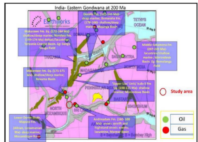
Figure 8: Source rocks of Eastern Gondwana with Oil and Gas fields 20
