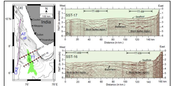
Figure 19: Illustrates the configurations of the seafloor and sub-basement within the Alleppey-Trivandrum Terrace Complex (ATTC) and surrounds, represented by (a) bathymetric contours, and (b) and (c) multichannel seismic reflection profiles along SST-17 and SST-16 37 .
