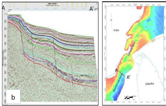
Figure 18: Seismic section across Mannar sub-basin depicting the Neogene compressional structures close to Comorin Depression 35
