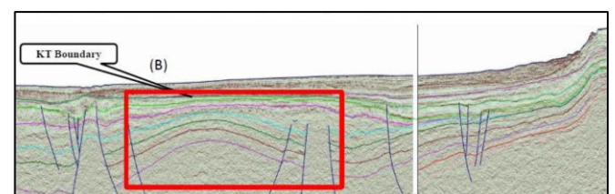
Figure 20: Seismic Profile across the Deep-water Basin (WNW to ESE) exhibiting Structural Inversion and Transpression within the Mesozoic 20
