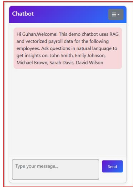
Figure 2: Chatbot
