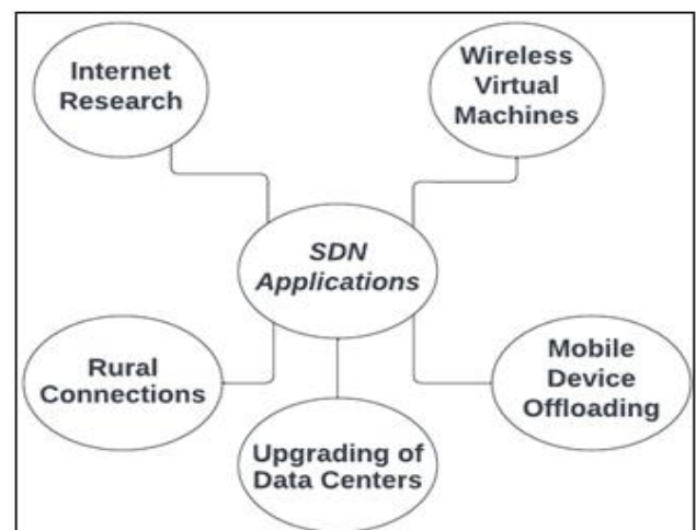
Figure 5: SDN Applications
