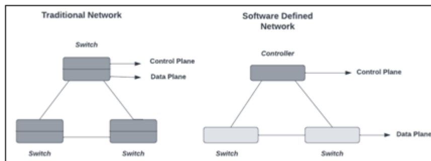
Figure 3: Traditional Network and SDN Network
