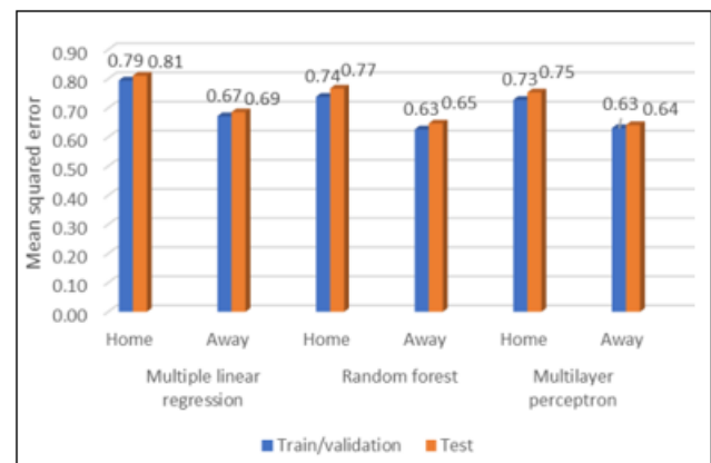
Figure 5: Each model's average MSE on the test and train/validation data
