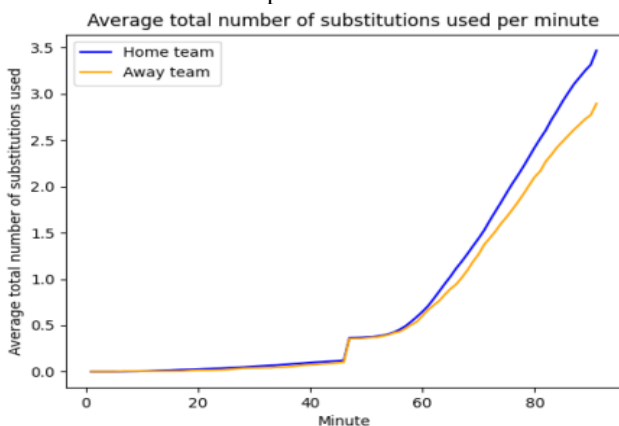
Figure 3: The total number of substitutions made by the home and away teams per minute
