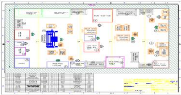
Figure 8: SLP layout
