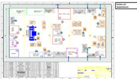
Figure 10: Final layout
