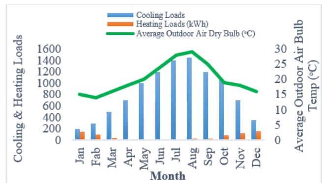
Figure 11: Cooling and Heating Loads with Average Outdoor Temperature – Existing
