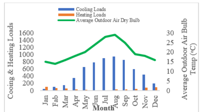
Figure 12: Cooling and Heating Loads with Average Outdoor Temperature – Proposed
