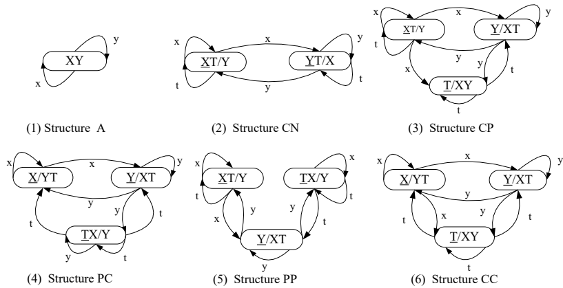
Figure 1: Six types of MCPs with corner equilibria
