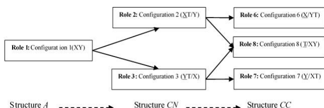
Figure 4: The evolution of the structures and role boundaries with the increase of \rho
