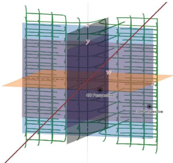
Figure 12: 4-dimensional plot for SD time in non-uniform motion
