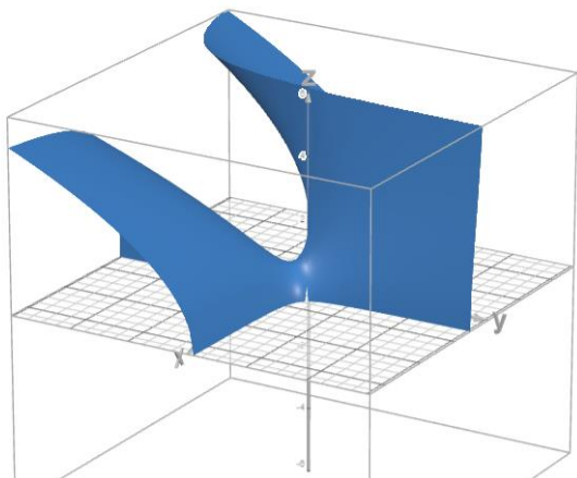
Figure 4: 3-dimensional projection of final SD time as per equation (9)
