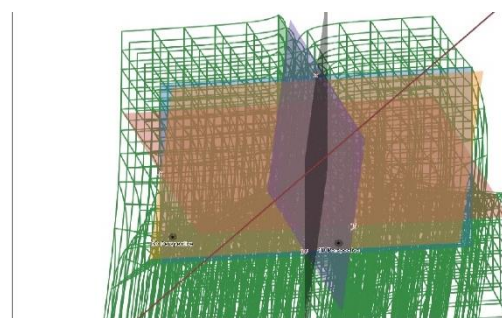
Figure 1: 4-Dimensional projection of final SD time as per equation (8)
