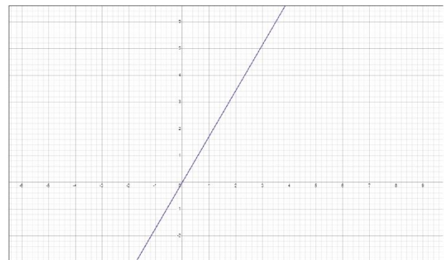
Figure 9: 2-dimensional plot of final SD displacement vs initial SD displacement
