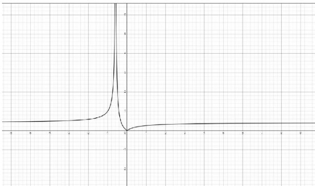
Figure 3: 2-dimensional projection of final SD time as per equation (8)
