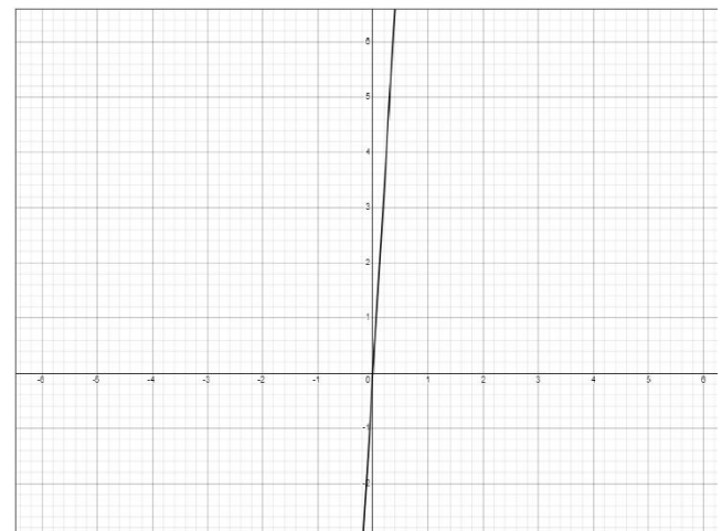
Figure 11: 2-dimensional plot between final SD velocity and initial SD velocity
