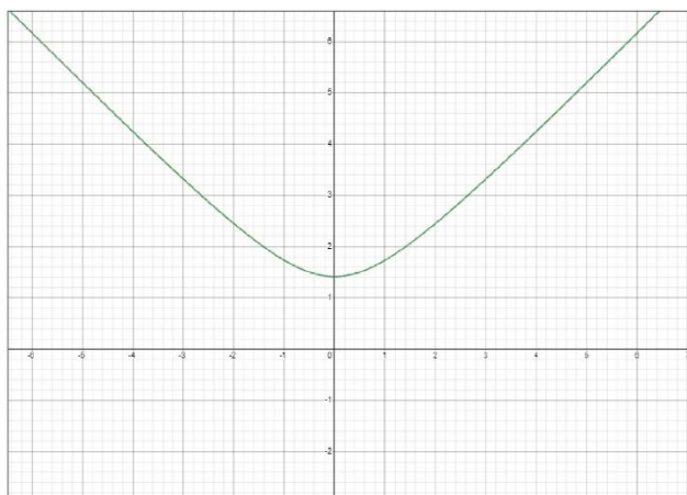
Figure 6: 2-dimensional projection of final SD time as per equation (10)
