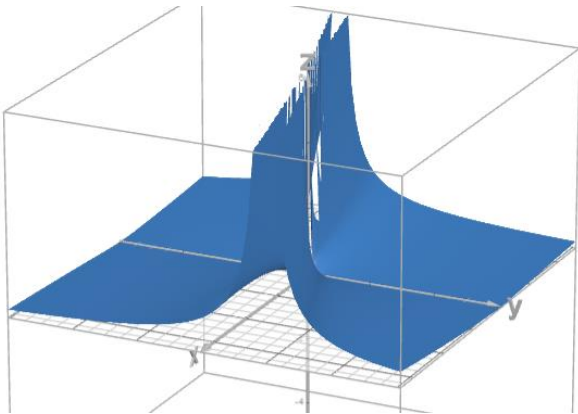
Figure 2: 3-dimensional projection of final SD time as per equation (8)
