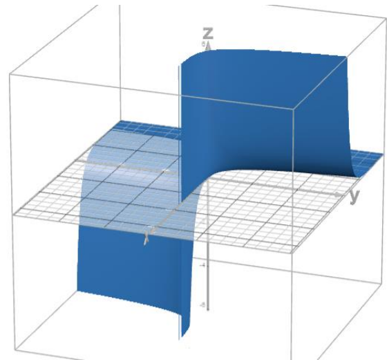
Figure 10: 3-dimensional plot for final SD velocity in terms of SD time and initial SD velocity
