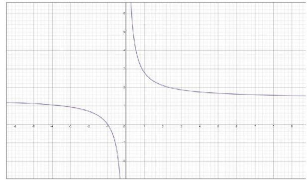
Figure 8: 2-dimensional plot of final SD displacement vs initial SD time
