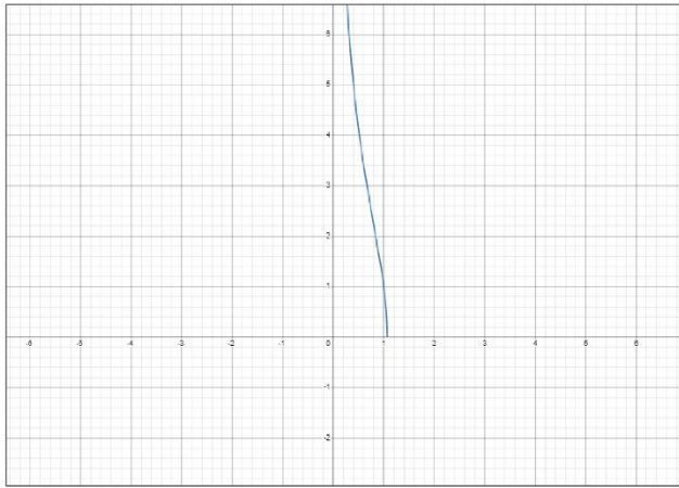
Figure 5: 2-dimensional projection of final SD time as per equation (9)
