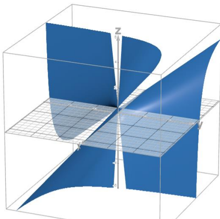
Figure 7: 3-dimensional plot of final SD displacement in terms of initial SD displacement and initial SD time
