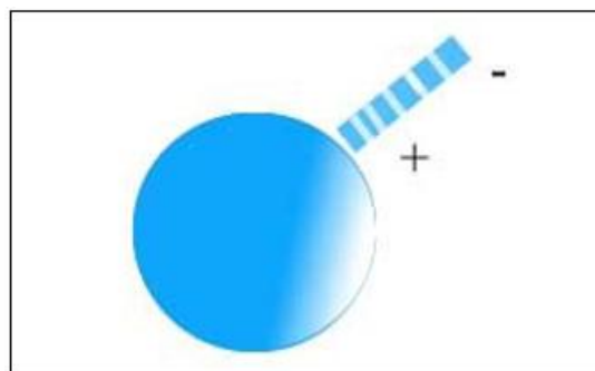
Pulses of electrical energy from electron are polarised
