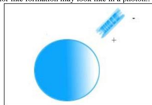
Solen Field take shape around pulses of energy forming a photon
