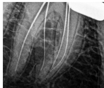
Figure 2: Working length radiograph (extra distolingual root)
