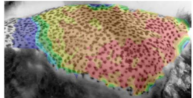
Figure 27: 12th max strain , no peripheral strain as noticed in the start
